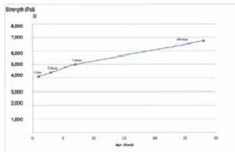
Fig. 1: Shotcrete typical strength gain.
